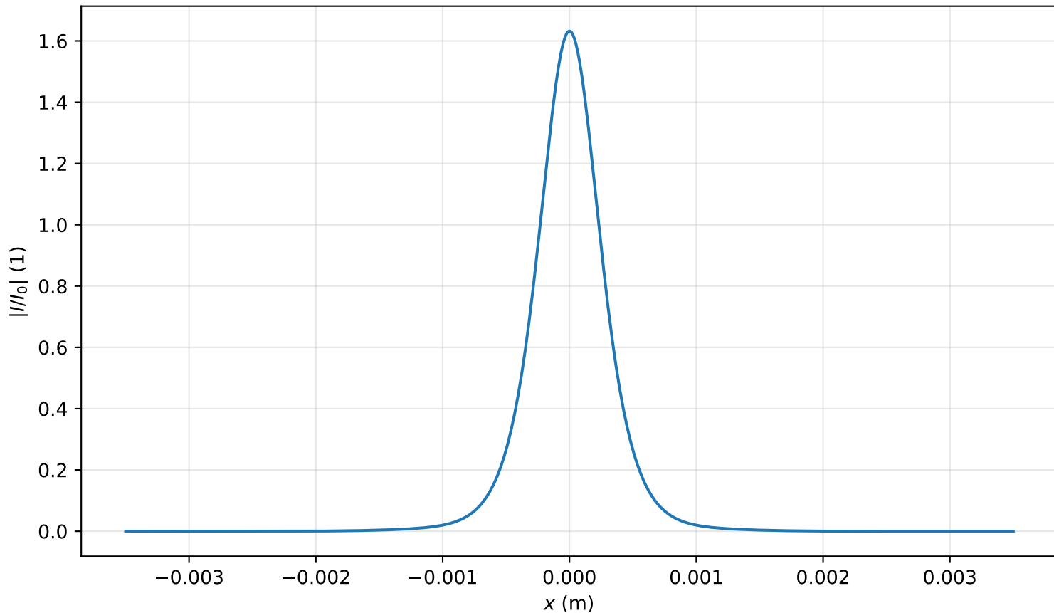
Intensity profile I(x, y = 0, z = 2.309m)/I_0 , P_{in}=0.9P_{cr} , artificial time
